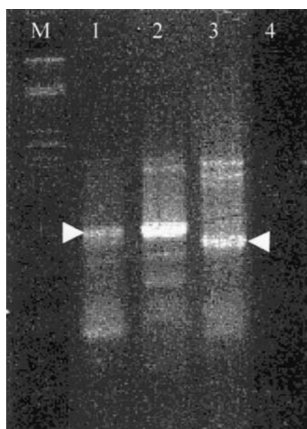
Figure 3. IC-RT-PCR amplification of PepMV and PVX genomic fragments using 'universal' primers for the potexvirus genus and \alpha -dsRNA antibody. M – molecular weight markers; 1 – extracts of PepMV-infected tomato fruits; 2 – extracts of PepMV-infected tomato leaves; 3 – extracts of PVX infected tobacco; 4 – negative control (healthy tobacco plant). White arrows indicate the main amplification bands.
