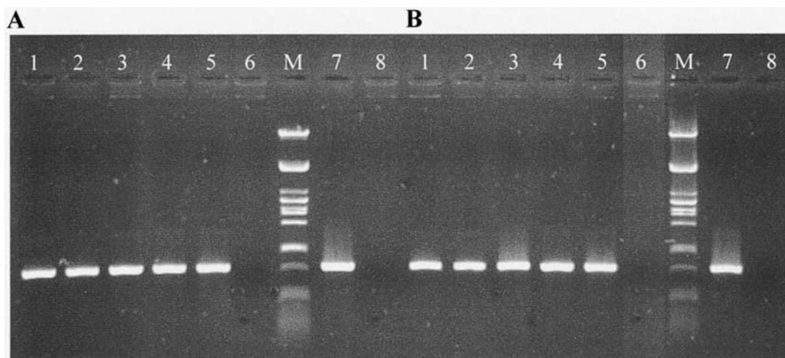
Figure 5. Specific amplification of an 835 bp fragment of samples infected with PepMV from different areas. 1 and 2 – IC-RT-PCR performed on extracts of Spanish samples infected with PepMV; 3 and 4 – IC-RT-PCR performed on extracts of British samples infected with PepMV; 5 – IC-RT-PCR performed on extracts of a Dutch sample infected with PepMV; 6 – negative control (healthy plant); M – molecular weight markers; 7 – PCR positive control (clone B DNA); 8 – PCR specificity control (PVX DNA). A – polyclonal PepMV antibody; B – monoclonal PepMV antibody.
