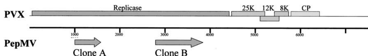
Figure 4. Relative position of PepMV amplified sequences reported in this paper with respect to the PVX sequence, based on nucleotide homology. The corresponding homology region for clone A in the PVX genome spans positions 1017–1635, and for clone B, positions 2865–3894.
